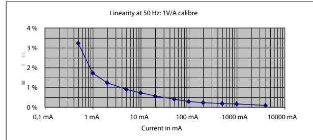
Linearity for AC
