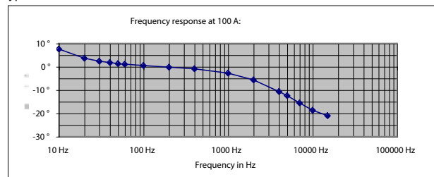
Phase shift typical
