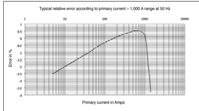
Linearity in AC
