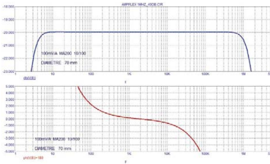
Frequency and phase responses (9)
