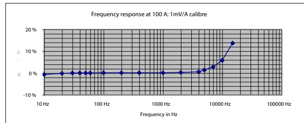
Typical error on measurement
