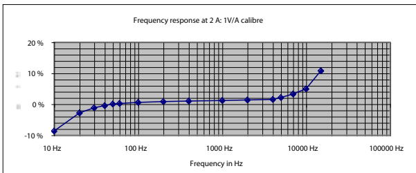
Typical error on measurement
