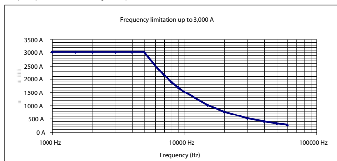
(6) Frequency limitation according to amplitude
